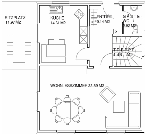
Erdgeschoss 8.21 x 9.41m
